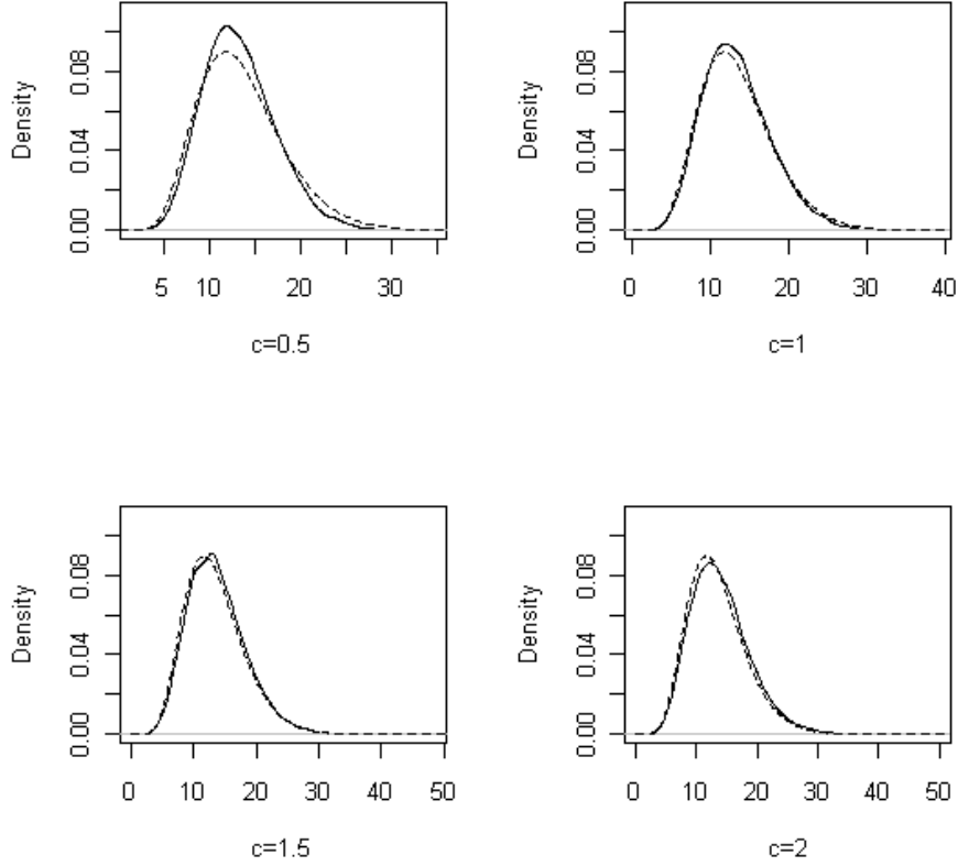
Figure 1: Exact distribution (solid line) versus asymptotic distribution (dashed line) of the test statistic with different bandwidth choices ( h = cn^{-1/4} )
